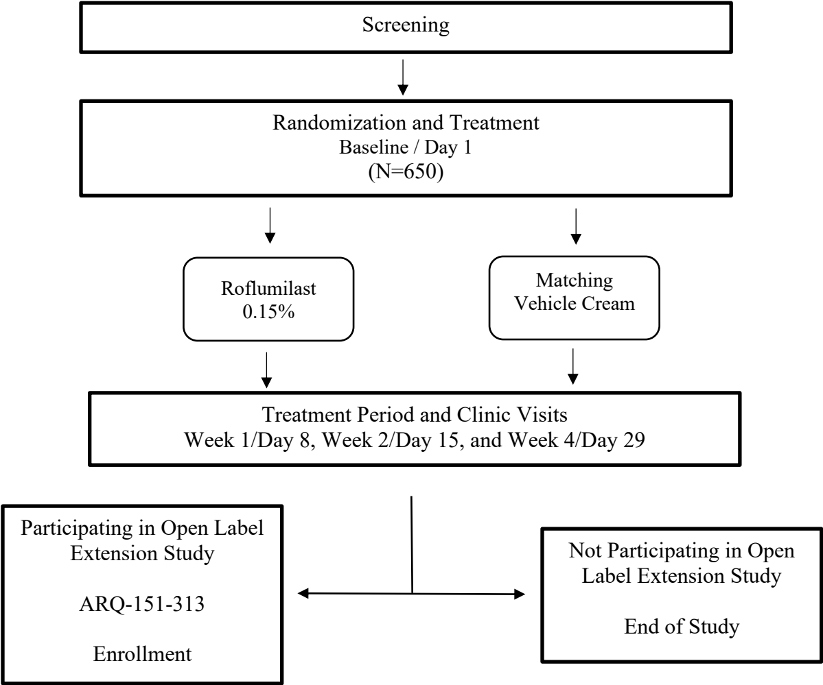
Figure 1 Study Schema
