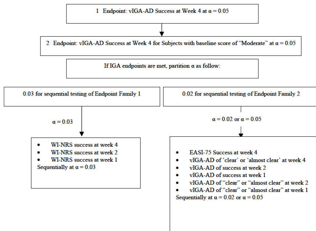
Figure 2 Multiple Testing Scheme
