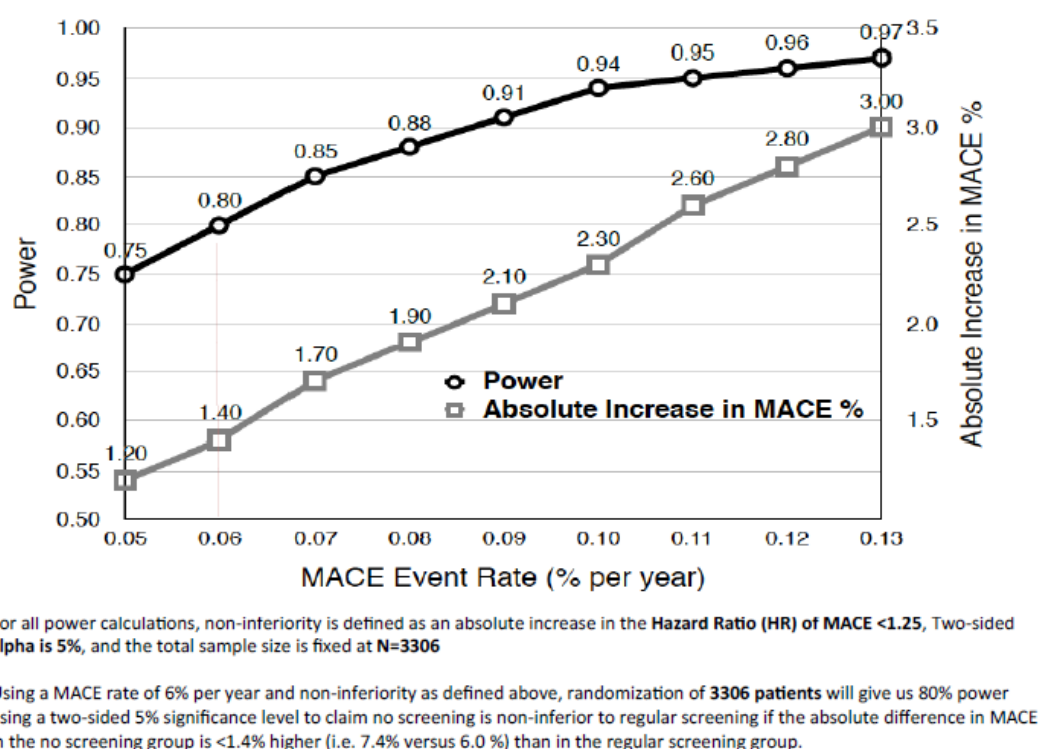
Figure 2: Study power for MACE rates
