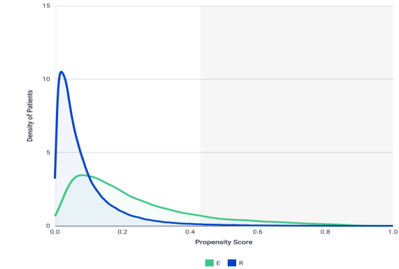
Figure 49: Pre-matching propensity score overlap
