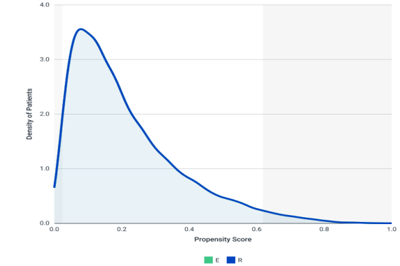
Figure 50: Post-matching propensity score overlap
