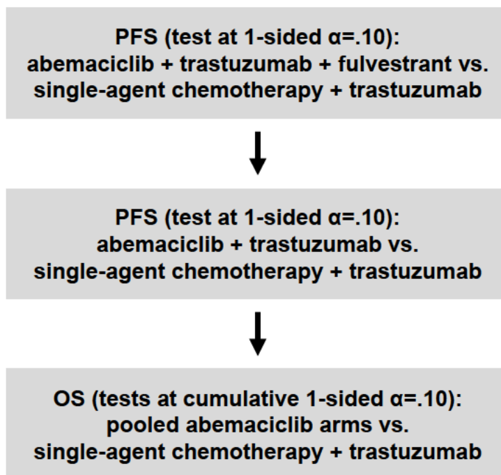
Figure JPBZ.12.1. Alpha spending for Study I3Y-MC-JPBZ.
