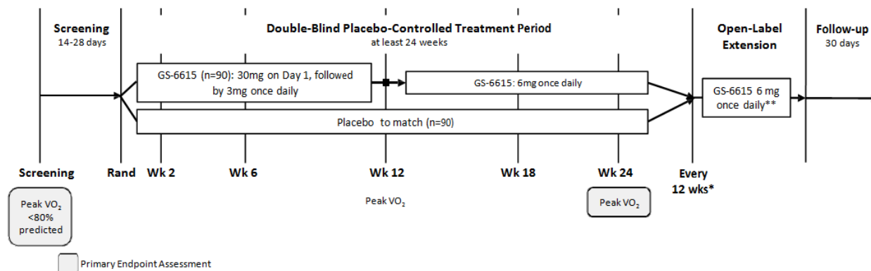
Figure 3-1. Study Schema
