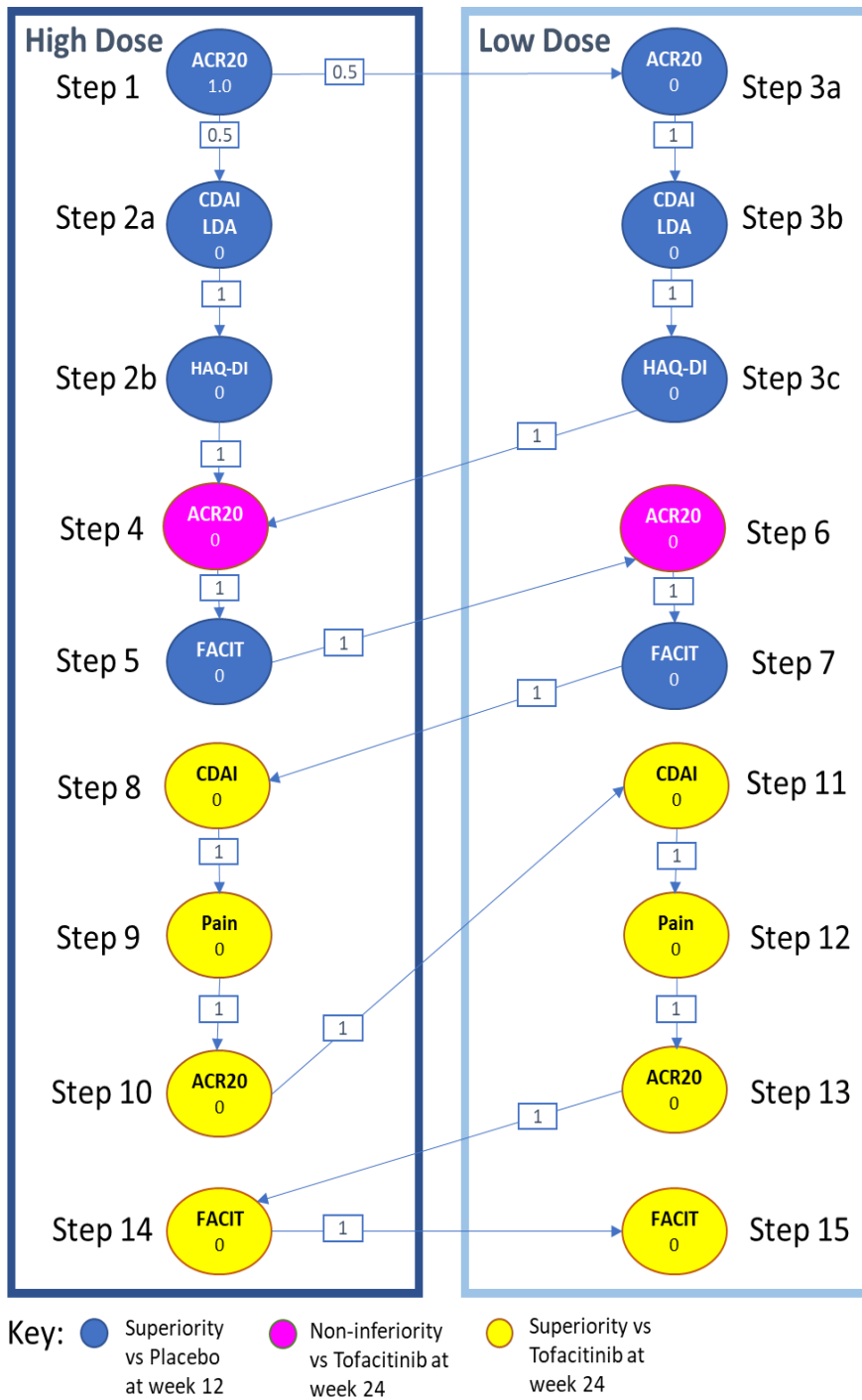
Figure 2 Graphical of the Multiple Testing Procedure
