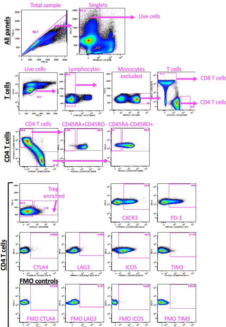
Figure 3: Gating hierarchy to identify lymphocyte subsets.
