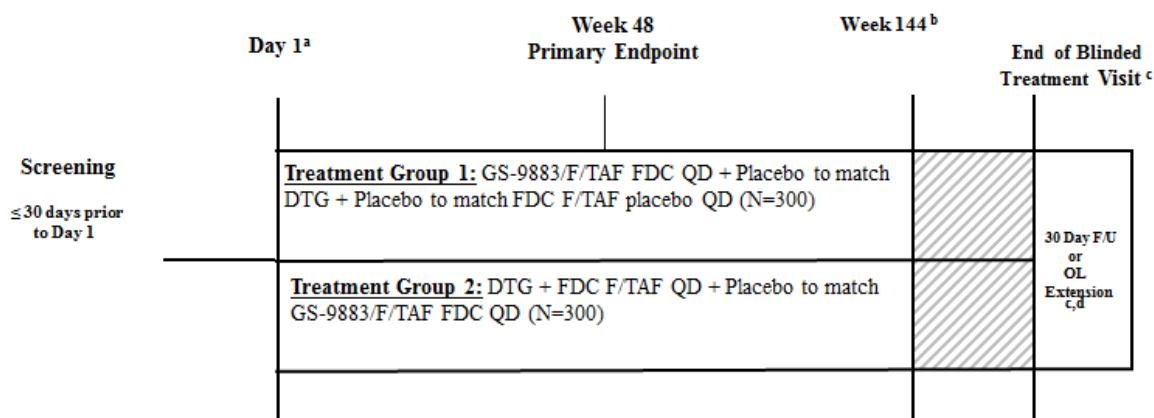
Figure 3-1. Study Schema
