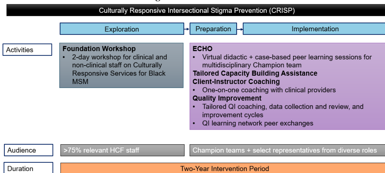
Figure 9: CRISP Model
