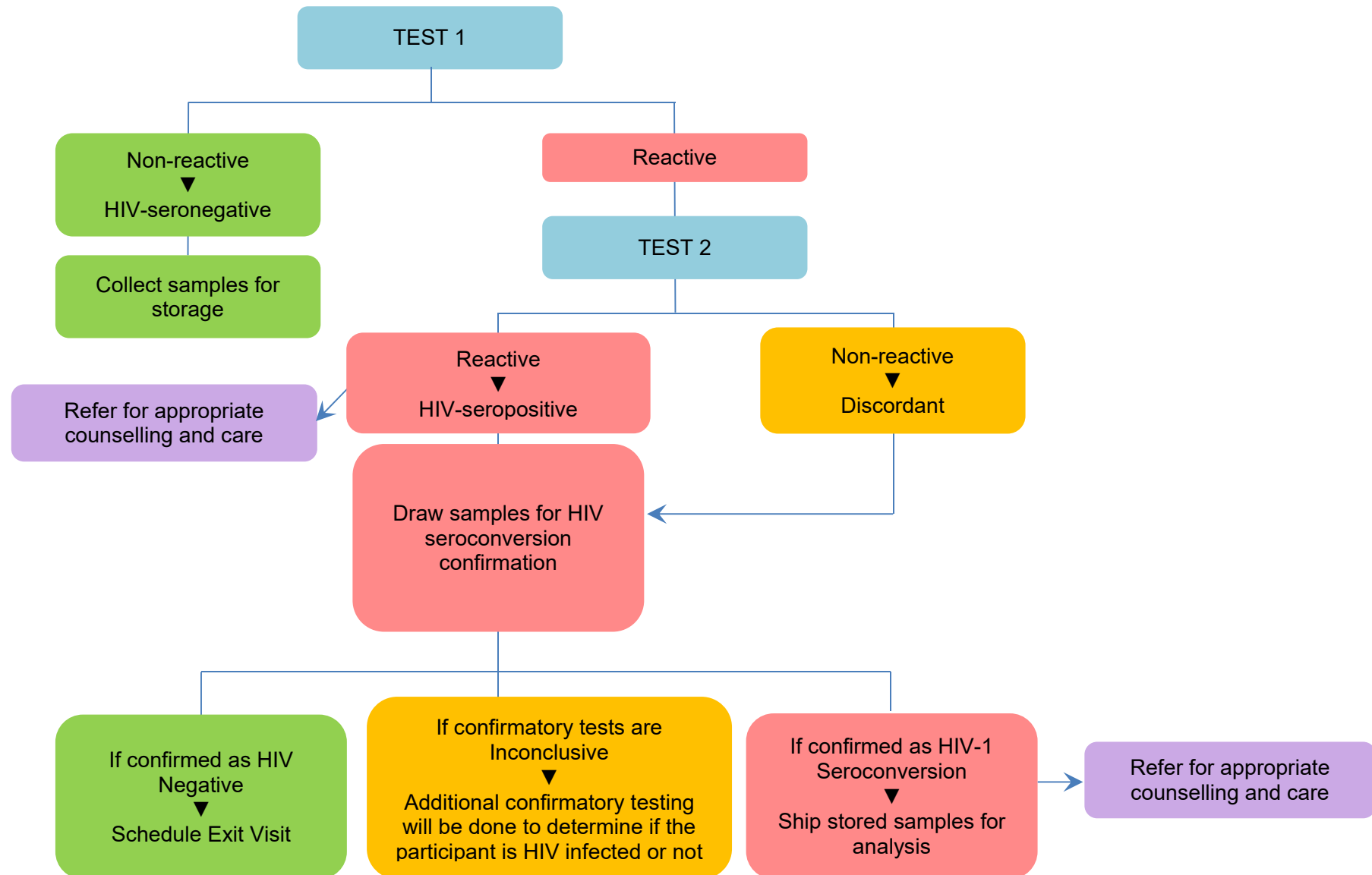
Figure 4: LPUV Algorithm
