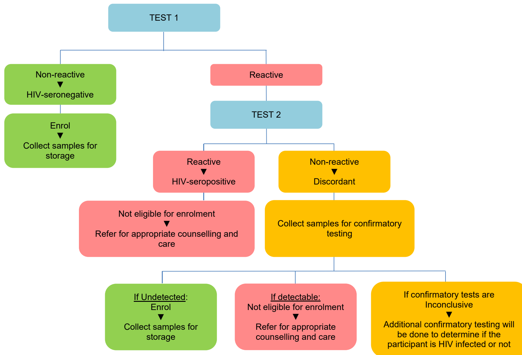
Figure 2: Pre-Enrolment Algorithm
