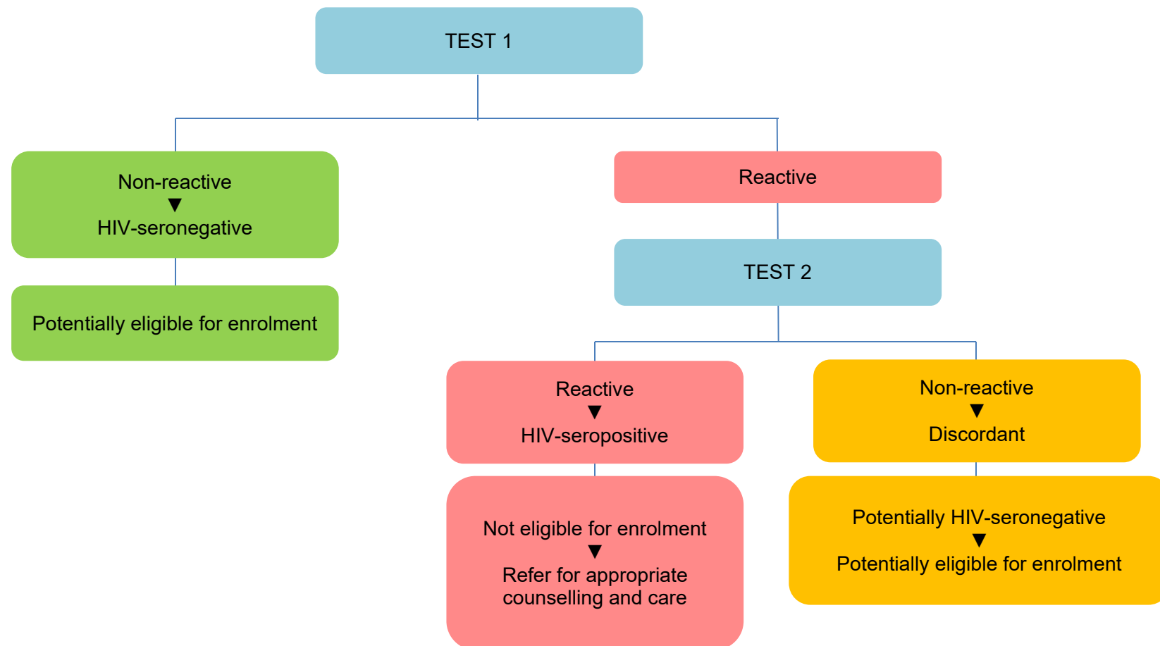
Figure 1: Screening Algorithm
