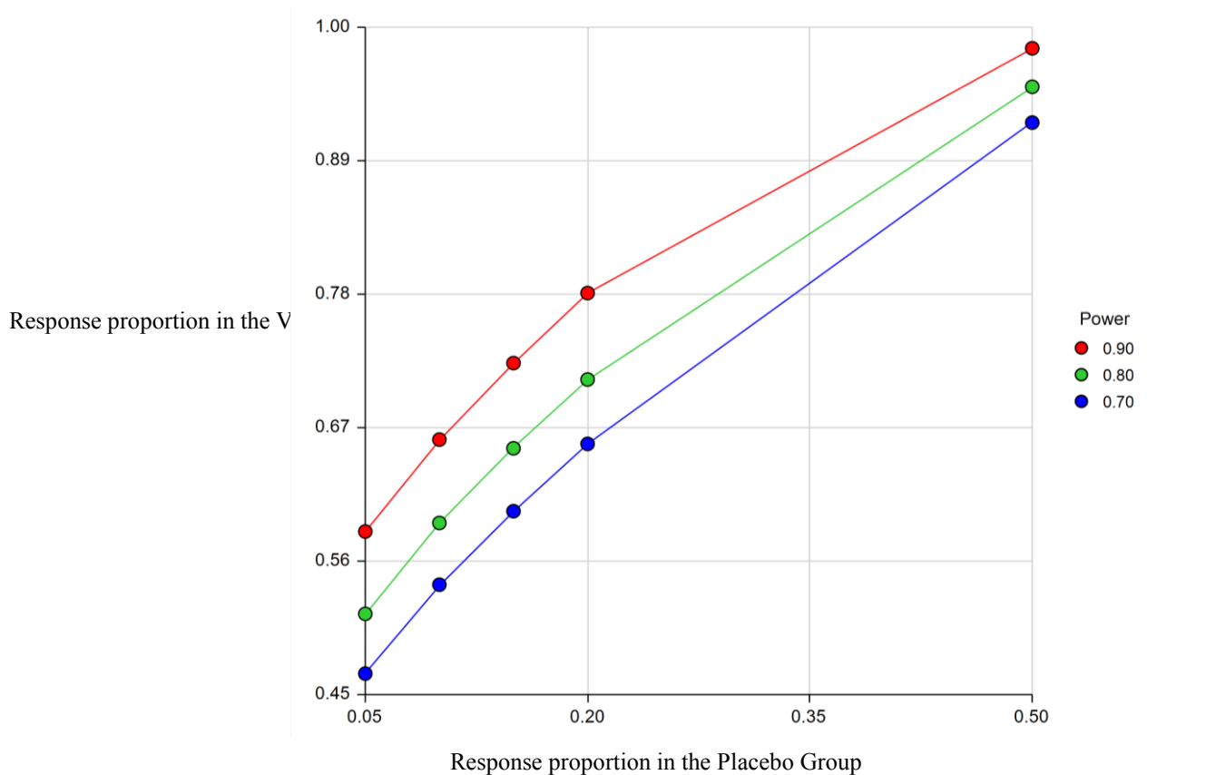
Figure 4: Power curves for comparisons between vaccine and placebo responses
