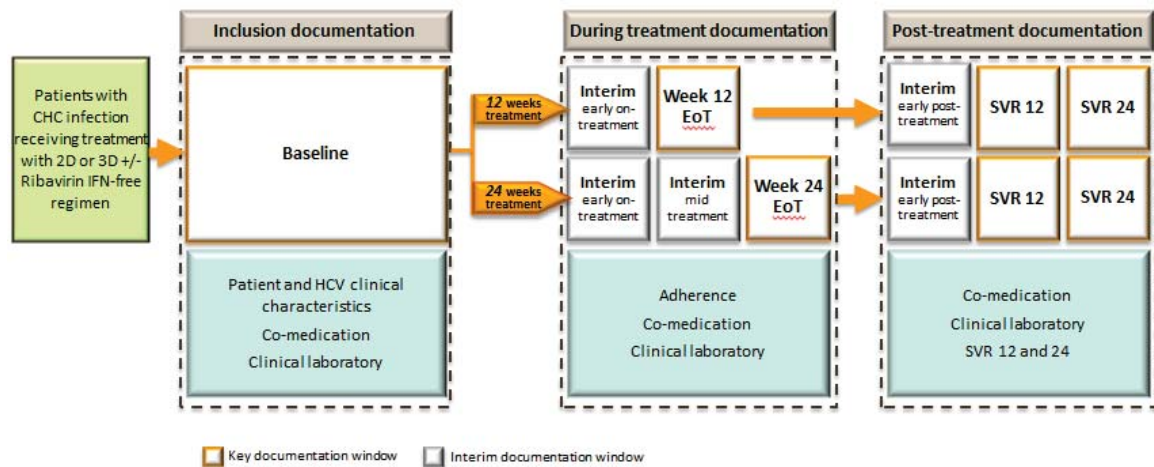
Figure 1 - Study Flowchart
